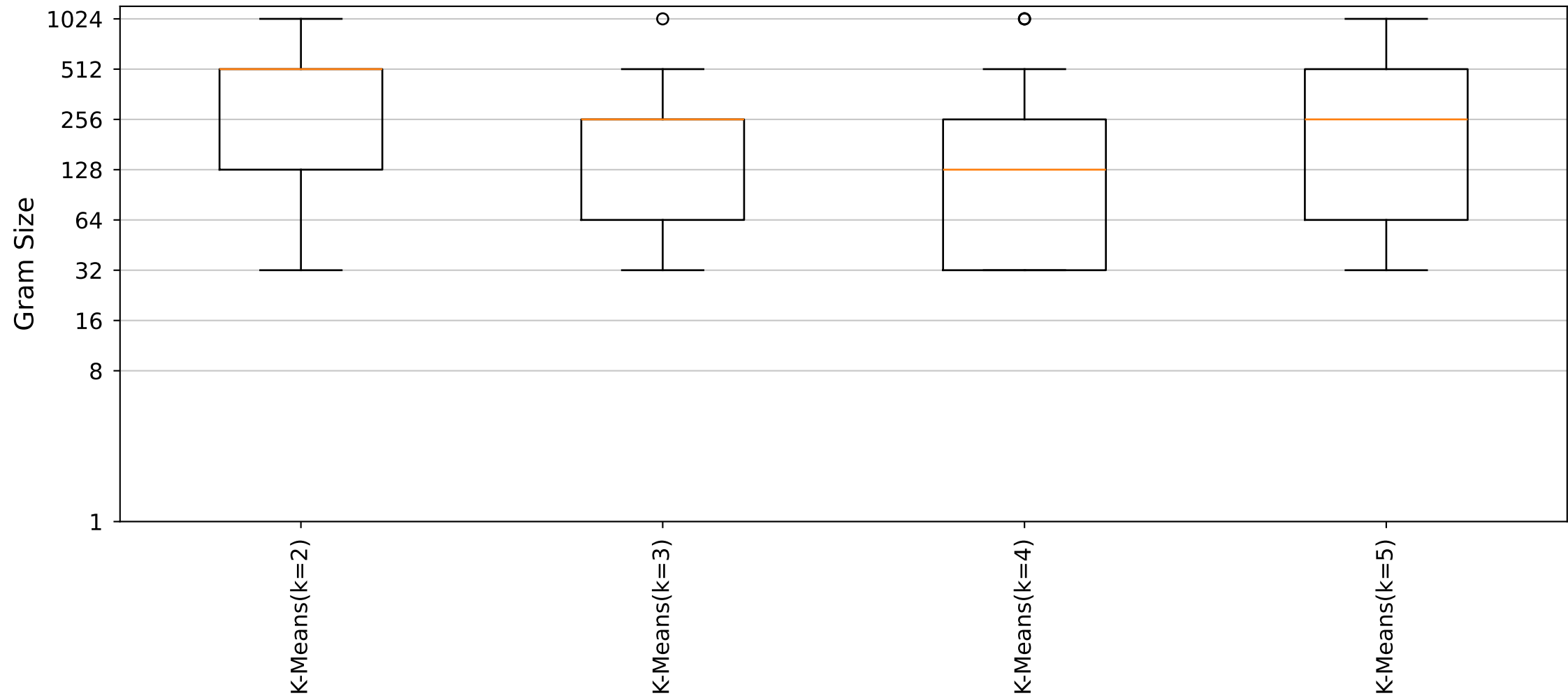
YARA Rules Gram Size Distribution (Cluster38_Size5 dataset)
